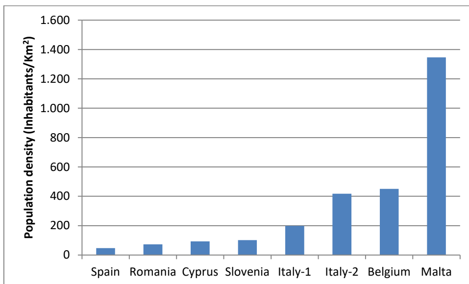
Figure 20. Population density.
