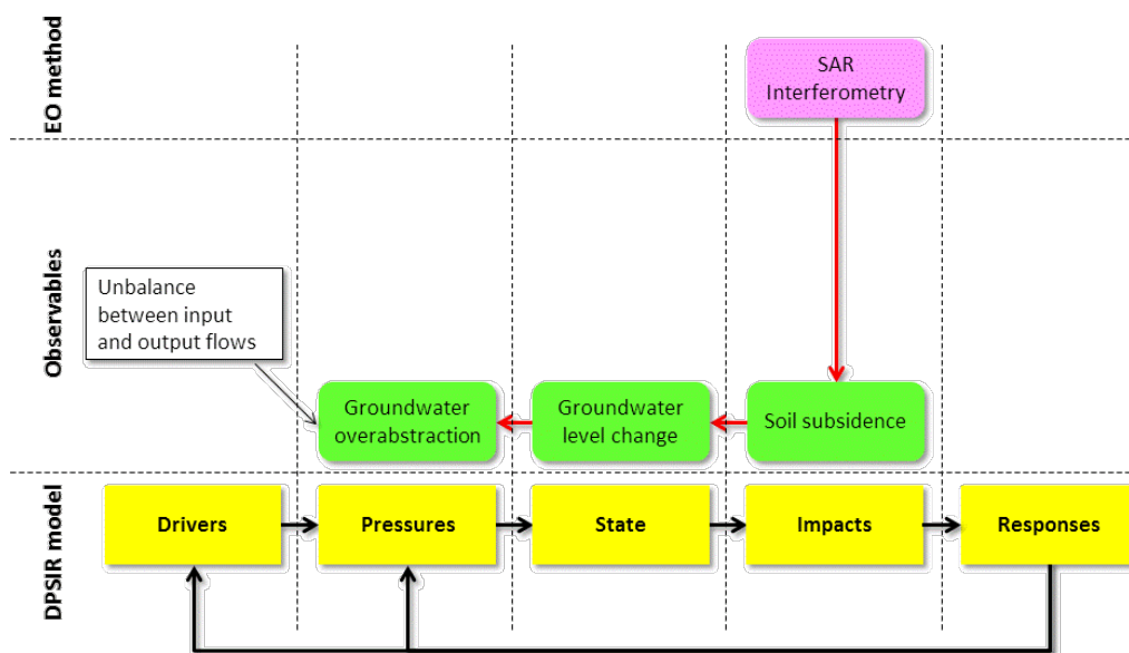
Figure 11. Taking as reference the DPSIR (Drivers, Pressures, State, Impacts, Responses) scheme, the EO method for the monitoring of the legal water over-abstraction provides the estimation of an environmental impact, i.e. the soil subsidence, caused by a change in the state of the groundwater level, caused in turn by an environmental pressure, i.e. the groundwater over-abstraction. Soil subsidence is a proxy of groundwater over-abstraction.
