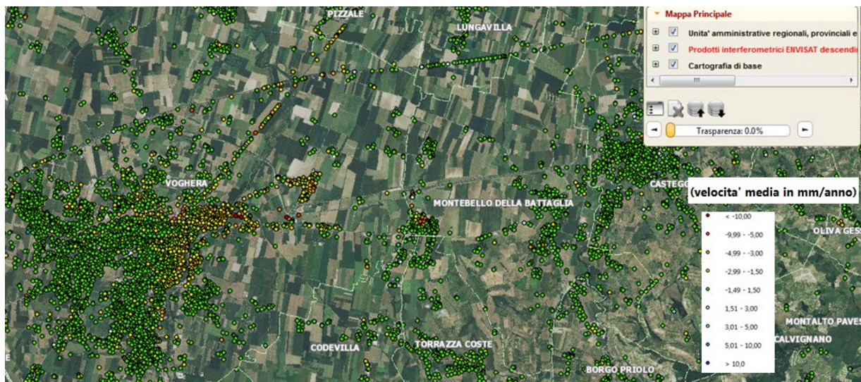
Figure 88: Extract, from the National Geoportal, of the SAR interferometric analysis from PST (ENVISAT series 2003-2008), in a portion of Oltrepò Pavese; single Permanent scatterers (PS) points are themed as a function of their average speed of displacement (mm/y) along the line of sight of the satellite during the period of analysis; yellow-red colors denote local subsidence.
