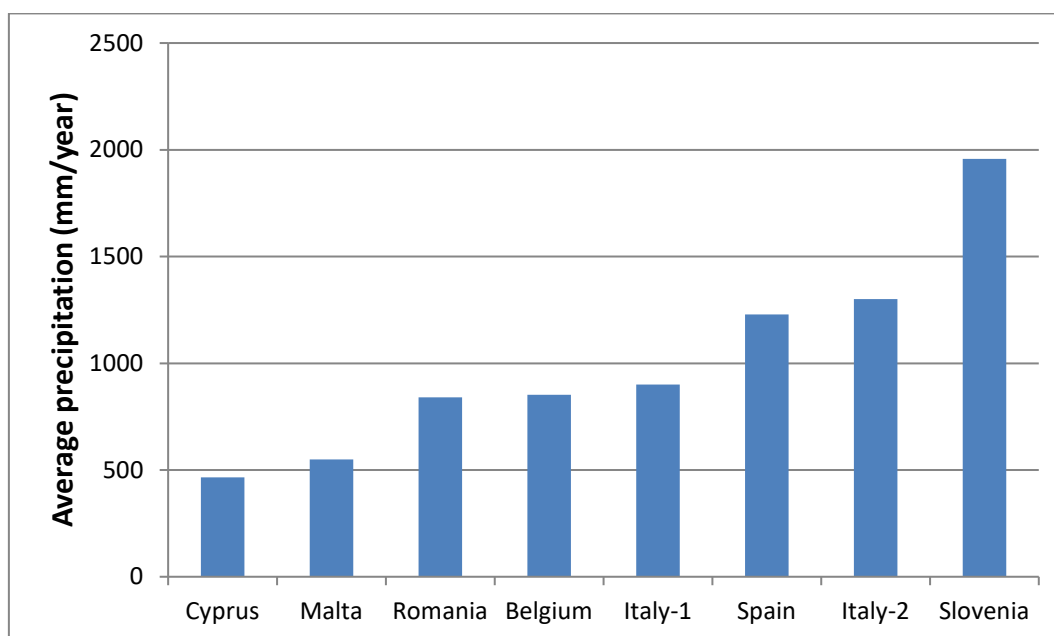
Figure 17. Average precipitations.
